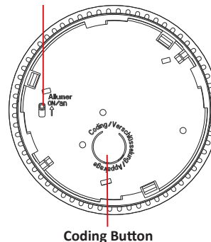
Power Switch
