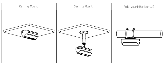
PFB110W Ceiling Mount Bracket
