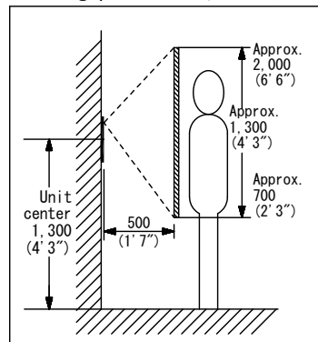
Mounting position 1,300mm (4' 3")
