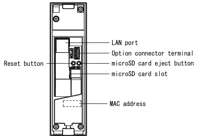
<Back view> Behind the Mounting frame
