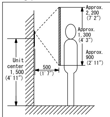
Mounting position 1,500mm (4' 11")
